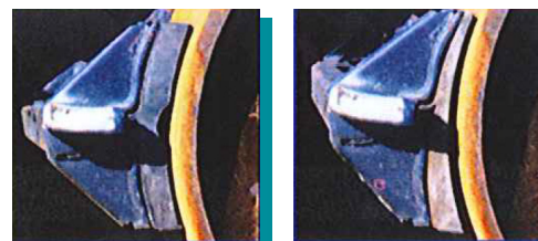
Brake beam droop causes shoe to contact wheel unevenly (right photo)
