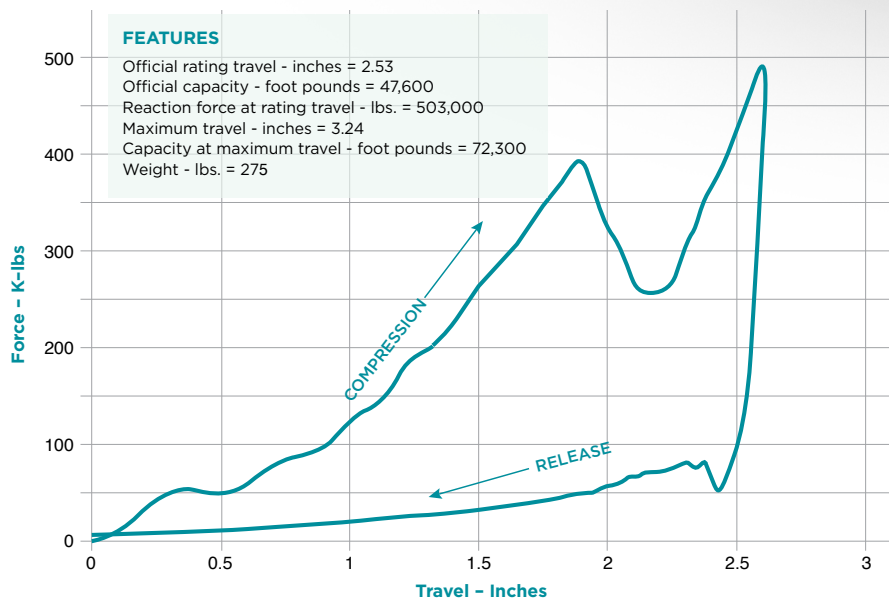
Endurance® 325 Typical Drop Hammer Performance Graph
